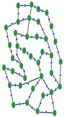
Amorphous Solids
